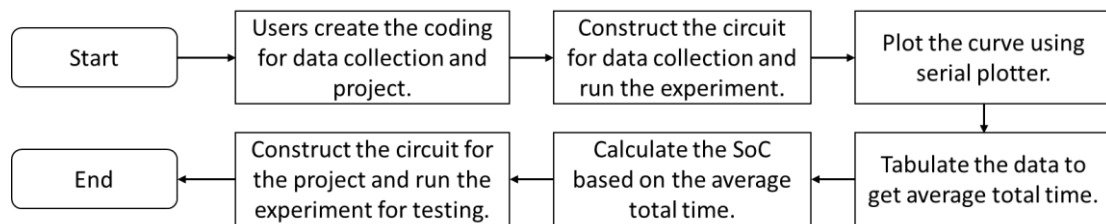
Figure 4: System flowchart
