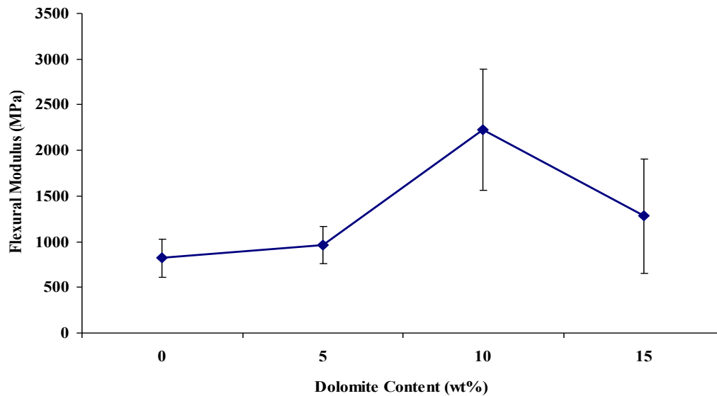
Figure 3 Flexural Modulus of PP and PP/Dolomite Composites
