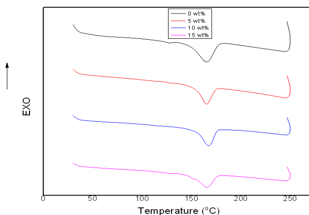
Figure 2 DSC Analysis Heating Scans of PP and PP/Dolomite Composites
