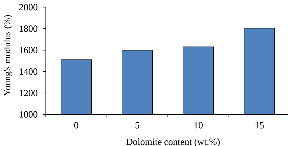
Figure 3 Effect of dolomite content on Young's modulus of PC/ABS 70/30 blends
