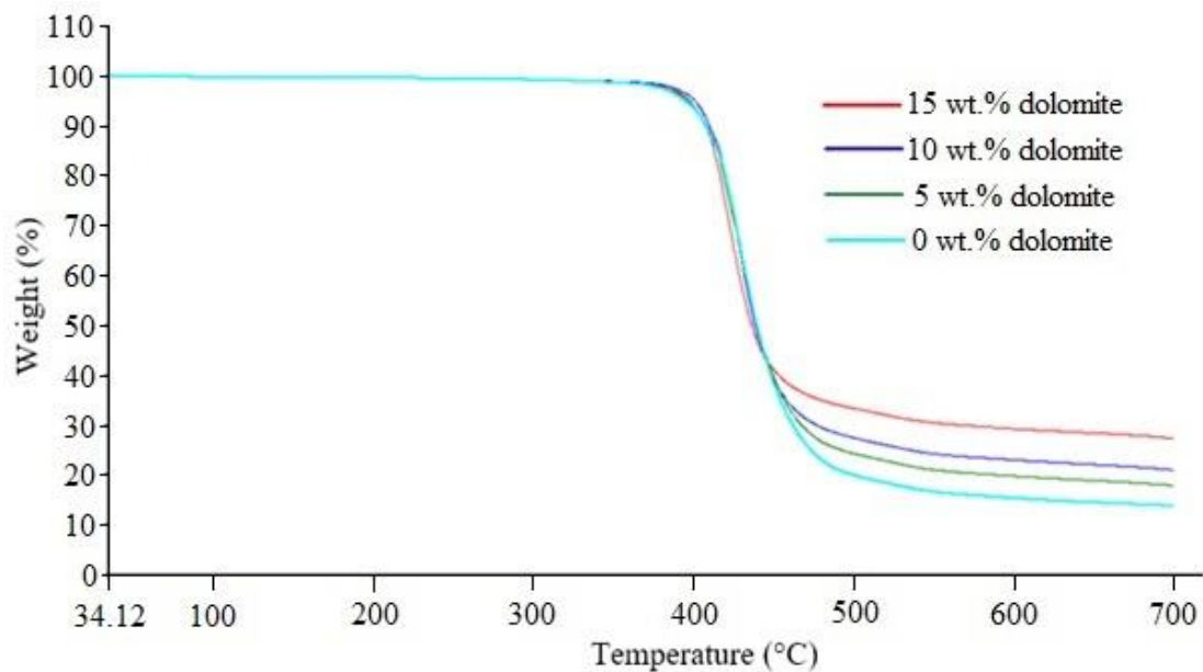
Figure 8 Curves of Thermogravimetric Analysis (TGA)
